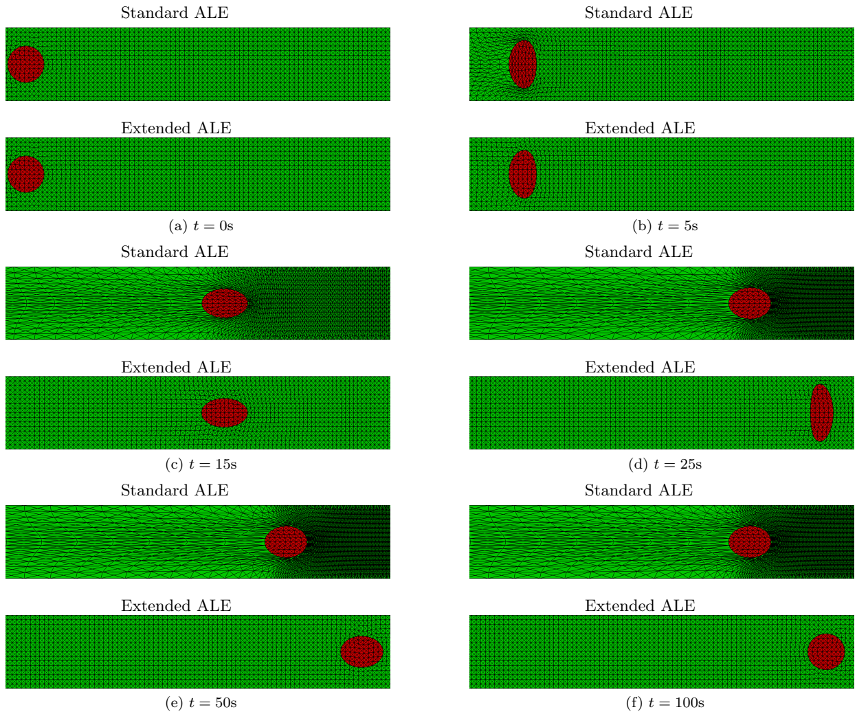
Figure 7: Beam position and mesh deformation for the periodic beam transported through a channel at (a) t = 0 s, (b) t = 5 s, (c) t = 15 s, (d) t = 25 s, (e) t = 50 s, (f) t = 100 s computed by the standard ALE method (top panel in each subfloat) and the Extended ALE method (bottom panel in each subfloat).
