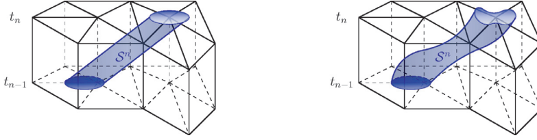
FIG. 1. Illustration of the local space-time triangulation \mathcal{Q}_h^S in one time slab. In the left picture we have a constant \mathbf{w} , and hence (2.13) is satisfied.
