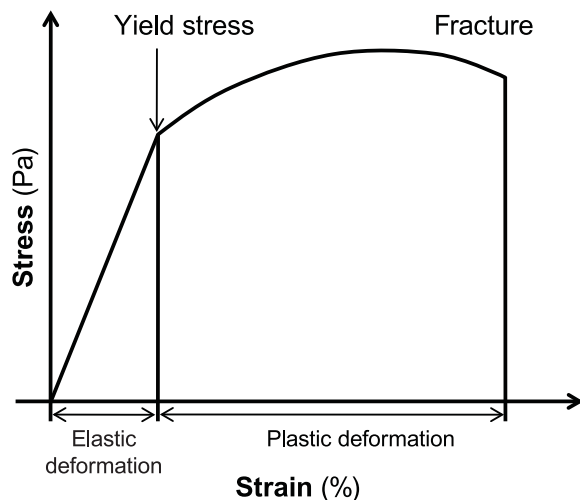
Fig. 1 Stress-strain relationship.
