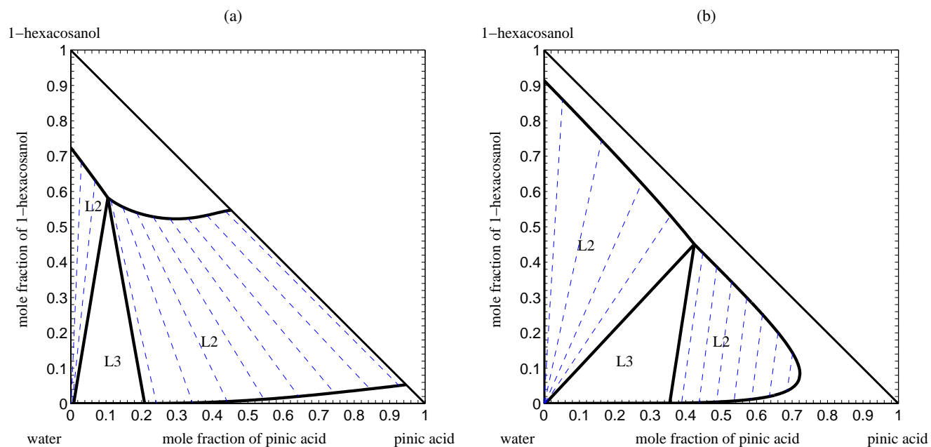
Fig. 6. Construction of the phase diagram for the system water/1-hexacosanol(X5)/pinic acid(X7) at 298.15 K with two different sets of UNIFAC parameters: (a) UNIFAC-Peng parameters, (b) UNIFAC-LL parameters
