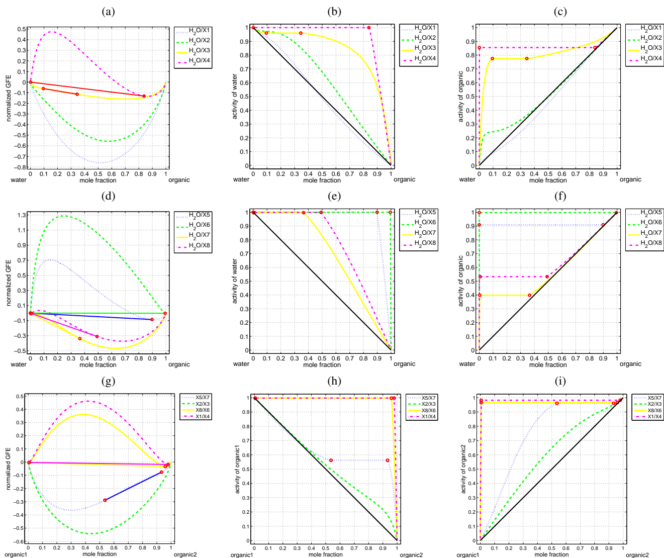
Fig. 1. Fig 1. Normalized GFE curves for all water/organic systems and two selected organic systems s_1/s_2 , and their respective activities. Equilibrium two phase solutions (if any) are marked with circle symbols. The solid (-) line represents the tie lines. Normalized GFE curves are plotted as a function of mole fraction of organic component s_2 for: (a) systems of water ( s_1 )/X[1-4] ( s_2 ) at 298.15K; (b) the activity of water in systems of water/X[1-4] and (c) activity of X[1-4] for the systems of water/X[1-4]. (d) Systems of water/X[5-8] at 298.15K. (e) The activity of water in systems of water/X[5-8] and (f) the activity of X[5-8]. (g) Systems of X5/X7, X2/X3, X8/X6, and X1/X4. (h) The activity of component s_1 for the s_1/s_2 system is shown in panel g, and (i) the activity of component s_2 for the s_1/s_2 system is shown in panel h.
