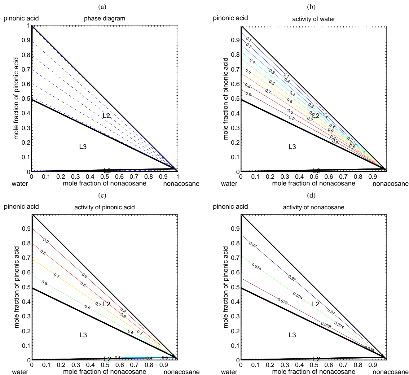
Fig. 4. Construction of the phase diagram for the system water/pinonic acid(X8)/nonacosane(X6) at 298.15 K with tracking of the presence of each distinct phase region. For each region the boundaries of which are marked with bold lines, the number of liquid phases at equilibrium is represented as L2 for two liquid phases and L3 for three liquid phases. (a) Liquid-liquid equilibrium prediction with two-phase tie lines represented by dashed lines. (b) Labels on the contours (—) indicate the value of the activity of water. (c) Labels on the contours (—) indicate the value of the activity of pinonic acid. (d) Labels on the contours (—) indicate the value of the activity of nonacosane.
