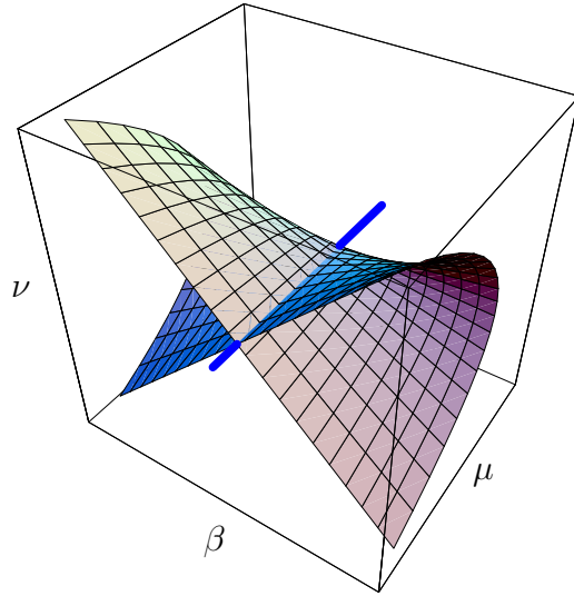
Figure 3: The Whitney umbrella \beta^2\mu + \nu^2 = 0 .
