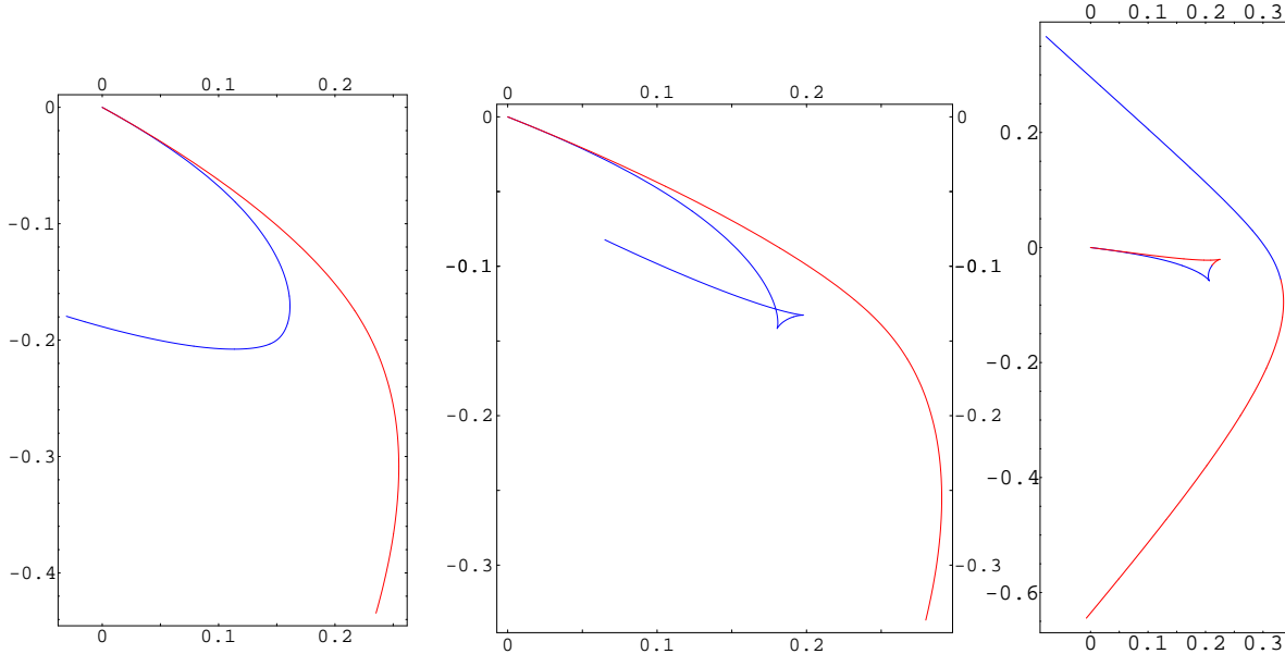
Figure 1: Resonance tongues with pocket- or flame-like phenomena near a degenerate Hopf bifurcation through e^{2\pi ip/q} in a family depending on two complex parameters. Fixing one of these parameters at various (three) values yields a family depending on one complex parameter, with resonance tongues contained in the plane of this second parameter. As the first parameter changes, these tongue boundaries exhibit cusps (middle picture), and even become disconnected (rightmost picture). The small triangle in the rightmost picture encloses the region of parameter values for which the system has four q -periodic orbits. These phenomena are explained in Section 5.
