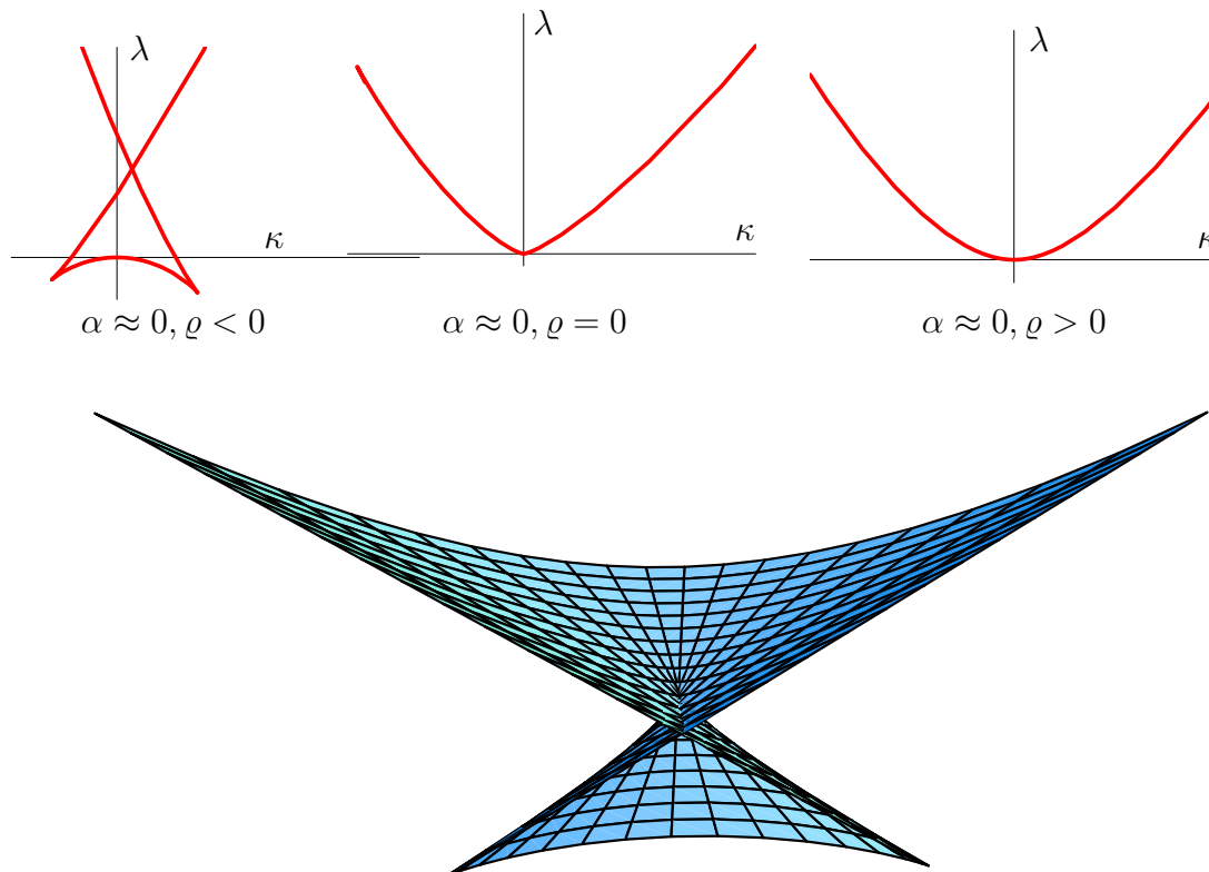
Figure 4: The discriminant set of the family \bar{Q}(u, \kappa, \lambda, \varrho, \alpha) = u^4 - u^5 + 2\alpha u^3 + \varrho u^2 + \lambda u + \kappa parametrized by (5.30), locally near 0 \in \mathbb{R}^4 . This surface is the product of the real line and a swallowtail, near 0 \in \mathbb{R}^4 . Top row: Cross-sections of D_{\bar{Q}} with planes (w, \alpha) = (w_0, \alpha_0) . Bottom row: Cross-sections of D_{\bar{Q}} with hyperplanes \alpha = \alpha_0 .
