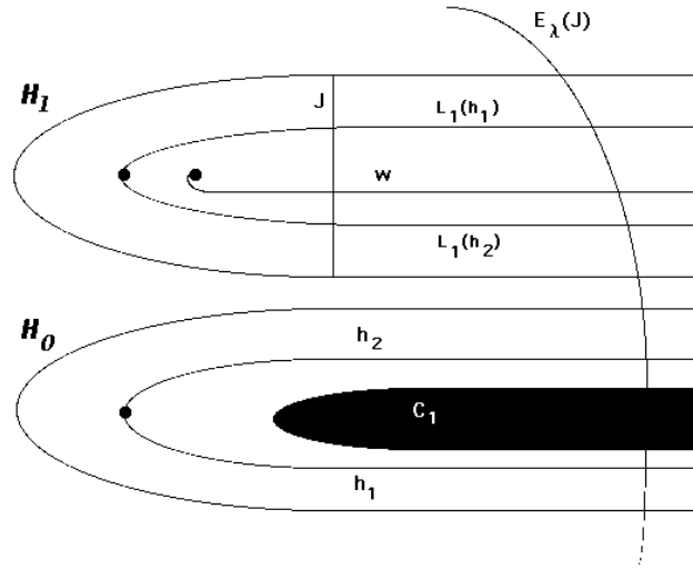
FIGURE 6. Inaccessibility of the itinerary \bar{1} .
