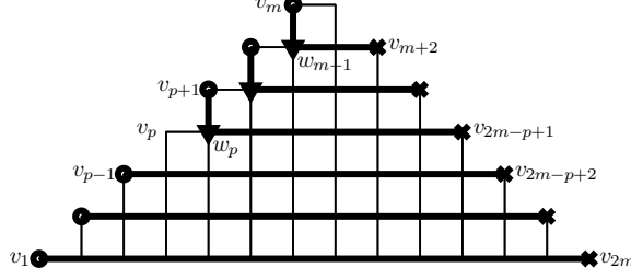
Figure B2. Connection for (Z; C) . Nodes in Z are \circ , nodes in C are \times . The paths are thick solid lines, edges not in the paths are narrow solid lines. Nodes at the intersections of vertical and horizontal path segments are \nabla .
