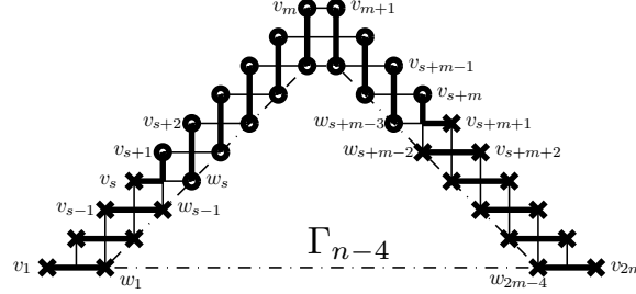
Figure A2. Induction step from \Gamma_{n-4} to \Gamma_n : connection between (P; Q) and (P'; Q') . Nodes in P and P' are \circ , nodes in Q and Q' are \times . Edges not in the connection are thin solid, edges in the connection are thick solid. Dash-dotted lines bound \Gamma_{n-4} (not actual edges).
