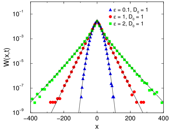
FIG. 1: Distribution of returns for a piecewise linear diffusion coefficient, Eq. (9), with D_0 = 1 . The shape of the distribution changes with the parameter \epsilon . Notice the special cases of \epsilon = 0 where the distribution is Gaussian, and of \epsilon = 1 where the distribution is exponential. The solid lines represent the analytical solution of Eq. (10), and the data points are the results of the random walk simulations with 10^6 independent walks, each one lasting a time t = 256 .
