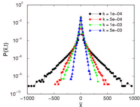
FIG. 8: Distribution of \bar{x} using the quadratic diffusion coefficient with dynamic consensus value. The tails of the distribution get heavier as k is decreased. This results were obtained using \epsilon = 1 , D_0 = 1 and t = 256 . The number of walks used was 2 \times 10^7 for k = 5 \times 10^{-3} and k = 10^{-3} , 4 \times 10^7 for k = 5 \times 10^{-4} and 5 \times 10^7 for k = 10^{-4} . Here again the solid lines serve as guides to the eye.
