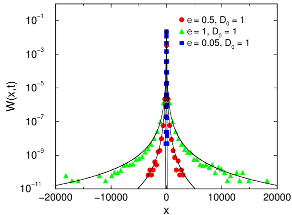
FIG. 2: Distribution of returns using the quadratic diffusion coefficient in Eq. (15). Note that the distribution is not exponential, but instead has fat tails. The solid lines represent the exact solution to Eq. (16), and the data points represent the results from the simulation. For \epsilon = 0.05 2 \times 10^7 walks were simulated, 5 \times 10^7 for \epsilon = 0.5 , and 6 \times 10^7 for \epsilon = 1 . The final time used in each case was t = 256 .
