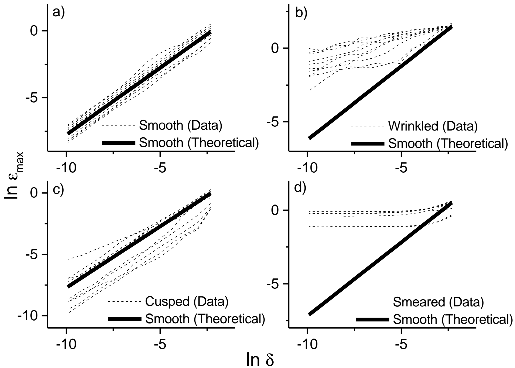
FIG 3 - P. So, et al., Limits to the Experimental Detection of Nonlinear Synchrony
