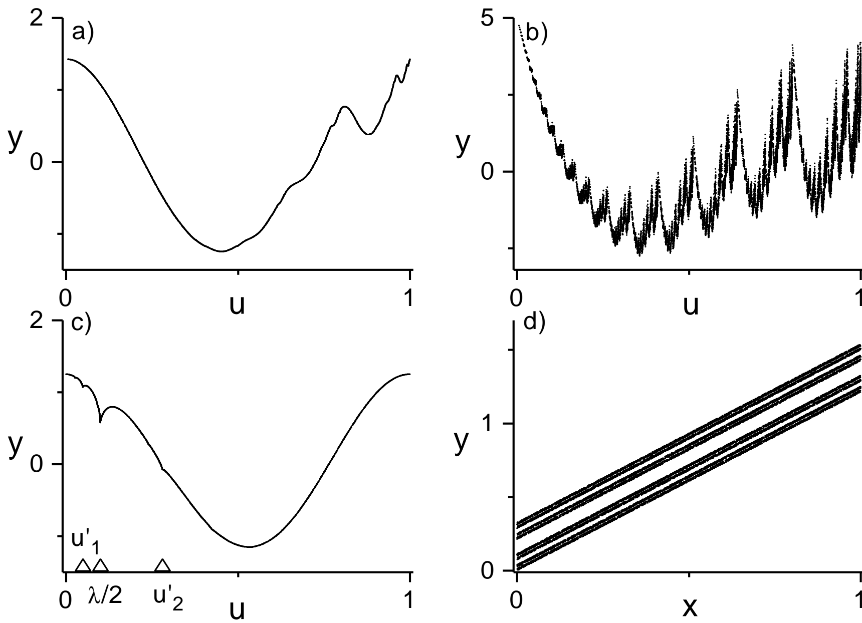
FIG 2 - P. So, et al., Limits to the Experimental Detection of Nonlinear Synchrony
