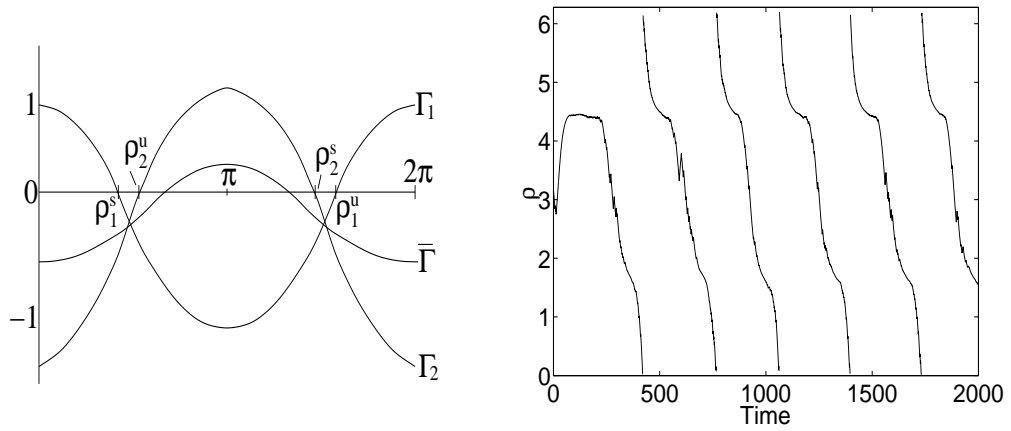
Figure 4: On the left are graphs of possible \Gamma functions whose average, \bar{\Gamma} , has a fixed point. However, because the convergence to the average is not sufficiently fast, the system will not phase lock. The evolution of \rho for such a system is shown on the right.
