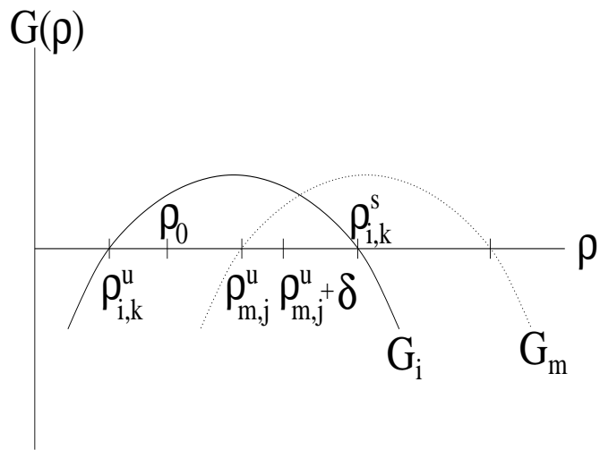
Figure 5: An illustration of the proof of proposition 7.2. For a sequence y_0, \dots, y_{N_1}, y_{N_1+1}, \dots, y_N the orbit of \rho_0 will first move past \rho_{m,j}^u + \delta at the N_1 -step, and past \rho_{i,k}^s at the N -th step.
