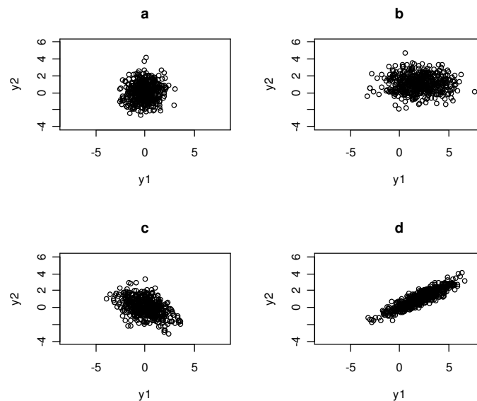
Figure 16.1: Simulated Bivariate Normal Data
