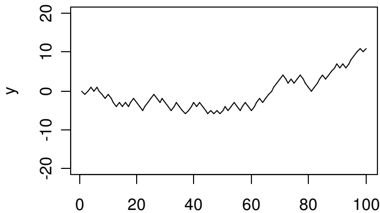
Figure 10-4: Simple Random Walk
