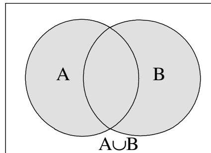
Figure 6-2: Union of Two Events
