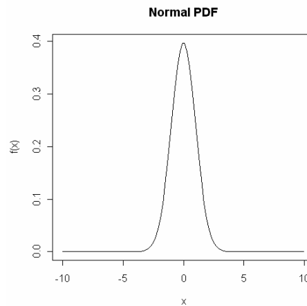
Figure 7-8: Univariate Standard Normal Distribution
