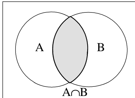
Figure 6-3: Venn Diagram of the Intersection of Two Events
