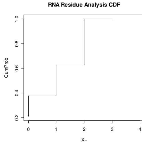
Figure 6-10: Cumulative Distribution Function for RNA Residue Analysis
