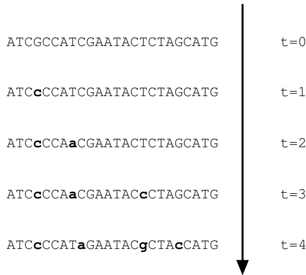
Figure 10-2: DNA Sequence Evolution as a Markov Process Over Time
