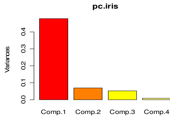
Figure 16.10: Screeplot of PC Analysis for Iris Versicolor
