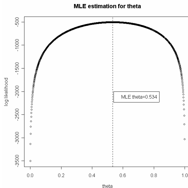
Figure 13-9: MLE for theta
