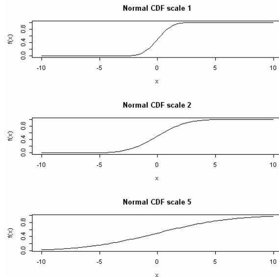
Figure 7-10: Normal Distribution CDFs with Different Scale Parameters
