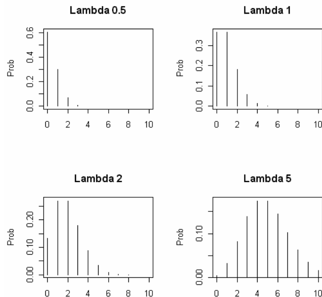
Figure 7-6: Poisson Distributions with Different Lambda Values
