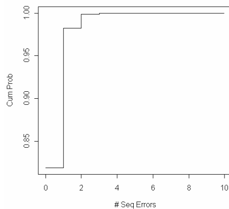
Figure 7-5: CDF for Poisson Model of Sequencing Errors with \Lambda = 0.2 .
