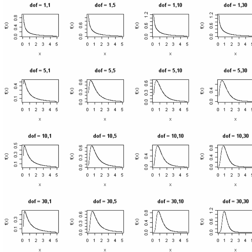
Figure 13-7: F distributions with varying df1 , df2
