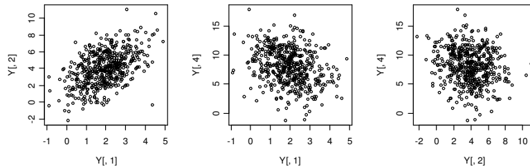
Figure 16.3. Two-dimensional marginal distributions: Scatterplots.
