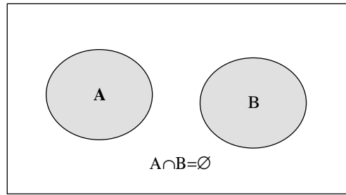
Figure 6-5: Intersection of Disjoint Events is the Null Set
