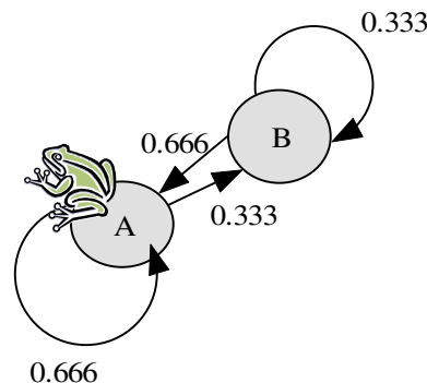
Figure 10-8: Transition Matrix for Frog's First 20 Jumps
