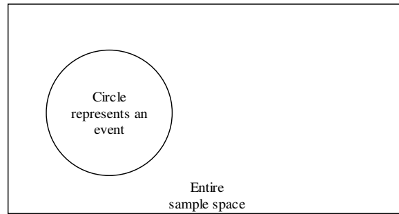
Figure 6-1: Basic Venn Diagram
