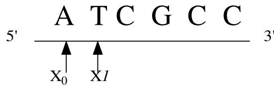
Figure 10-3: 5' to 3' Nucleotide Dependencies as a Markov Process
