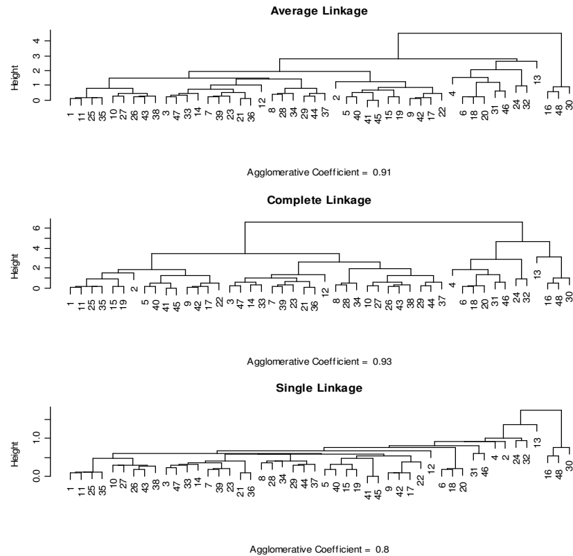
Figure 16.17. Agglomerative Clustering of Sleep Data using Three Different Linkage Methods
