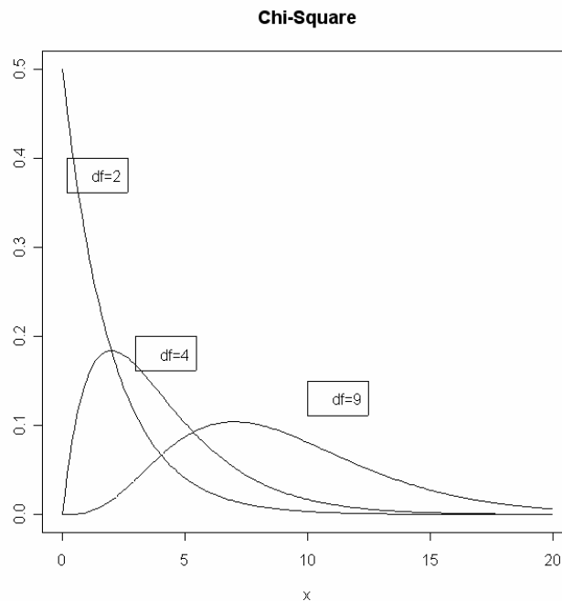
Figure 13-6: Chi-Square Distribution with 2, 4, and 9 Degrees of Freedom
