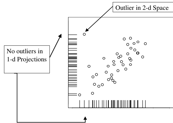
Figure 16.8: Masking of Outlier in Projections
