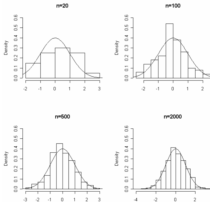
Figure 13-1: Effect of Sample Size on Approximating the Underlying Distribution
