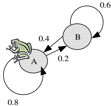
Figure 10-6: Transition Probabilities for Frog's First Move
