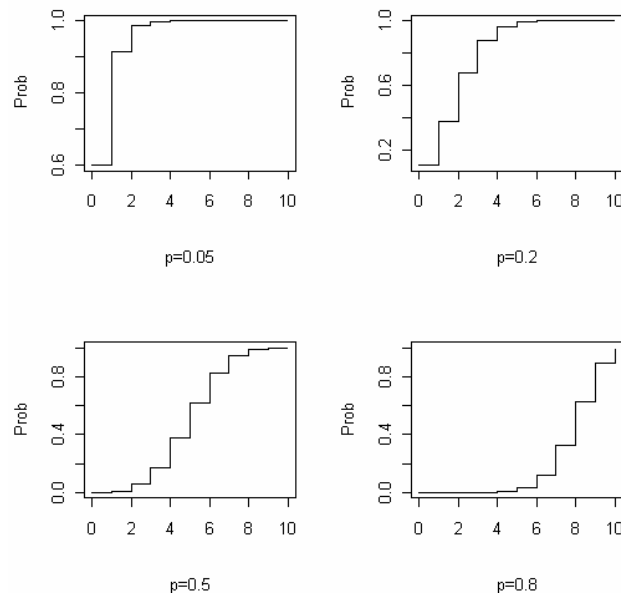
Figure 7-3: Binomial CDFs Using Different Values of p
