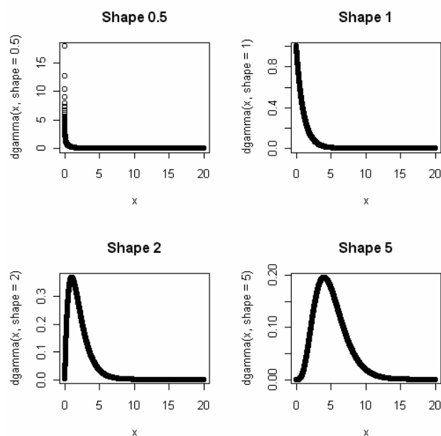
Figure 6-12: Altering a Shape Parameter with Other Parameters Held Constant
