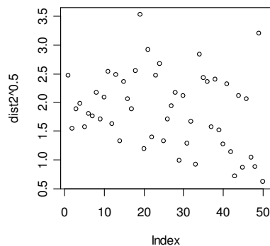
Figure 16.9 Multivariate distances of Iris Versicolor Data
