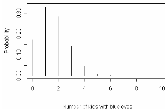
Figure 7-1: Example of a Binomial Distribution, p=0.16
