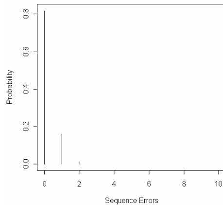
Figure 7-4: Poisson Distribution, \Lambda = 0.2 .
