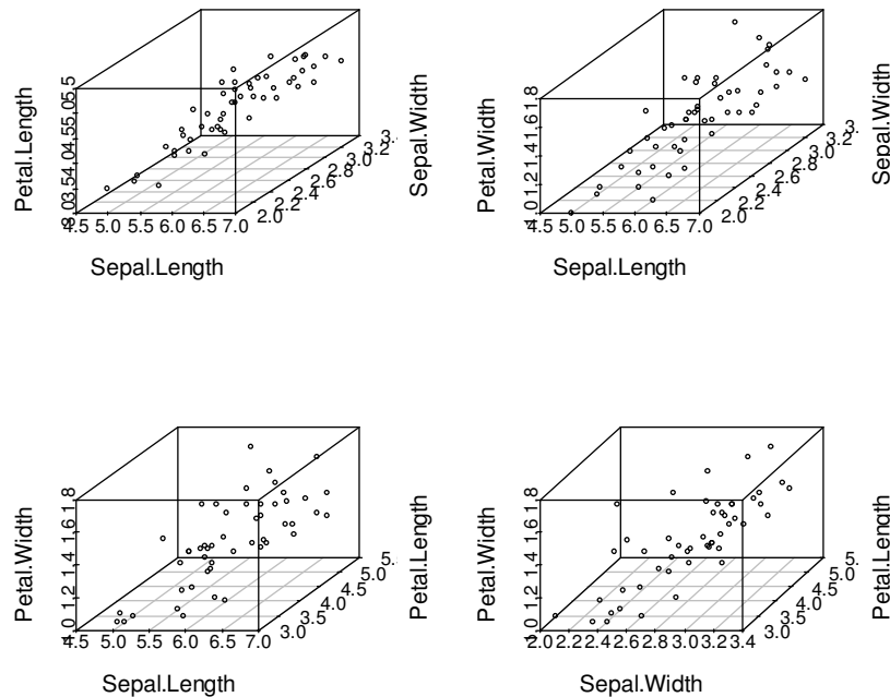
Figure 16.7: 3-d Point Clouds of Iris Versicolor Data
