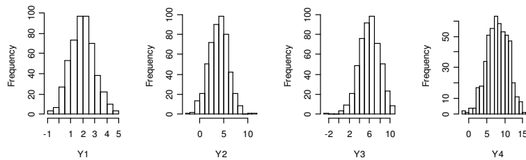
Figure 16.2. One-dimensional marginal distributions: Histograms
