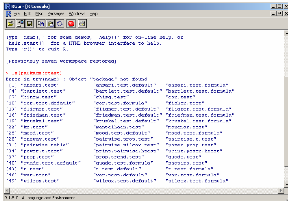
Figure 14-2: Contents of package ctest
