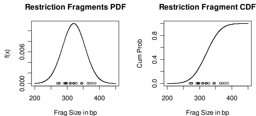
Figure 7-11: PDF and CDF for restriction fragment data
