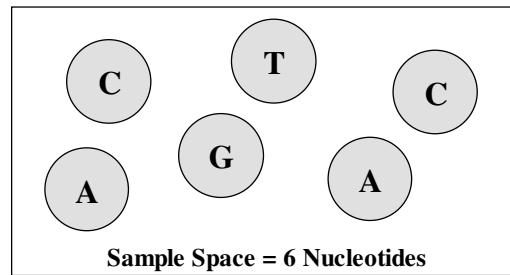
Figure 6-7: Sample Space for 6 Nucleotides
