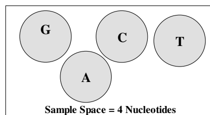
Figure 6-6: Sample Space for 4 Nucleotides
