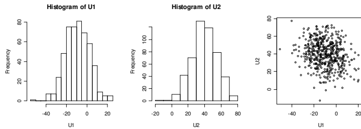
Figure 16.4: Distributions of Linear Combinations of Normal Variates
