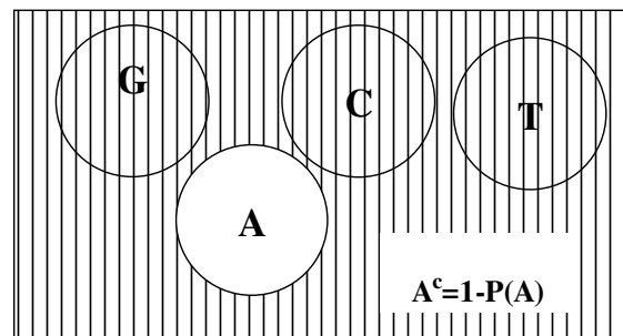
Figure 6-8: The Complement of A is everything in the Sample Space Except the Event A
