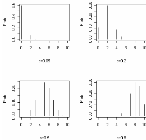
Figure 7-2: Illustrating the Effect of Changing the Value of p in the Binomial Distribution
