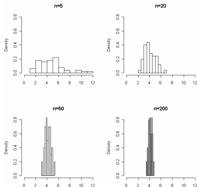
Figure 13-3 Illustrating the Law of Averages
