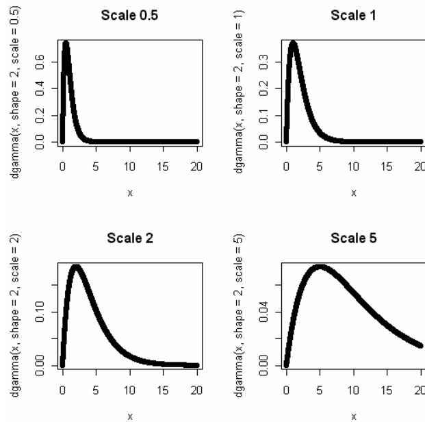
Figure 6-13: Altering a Scale Parameter with Other Parameters Held Constant
