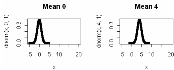
Figure 6-14: The Effect of changing the Location Parameter
