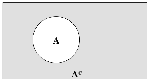
Figure 6-4: Venn Diagram of the Complement of an Event
