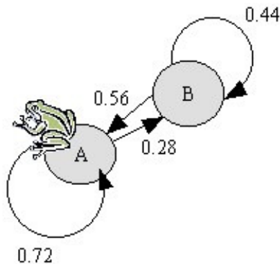
Figure 10-7: Transition Probabilities for Frog's First Two Moves
