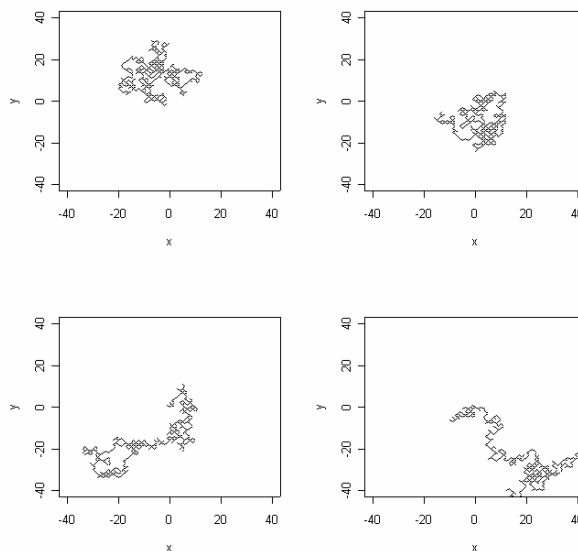
Figure 10-5: Two Dimensional Random Walk Outcomes (same simulation)
