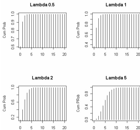
Figure 7-7: Poisson CDFs with Different Lambda Values
