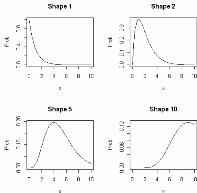
Figure 7-12: Gamma distributions with different shape parameters
