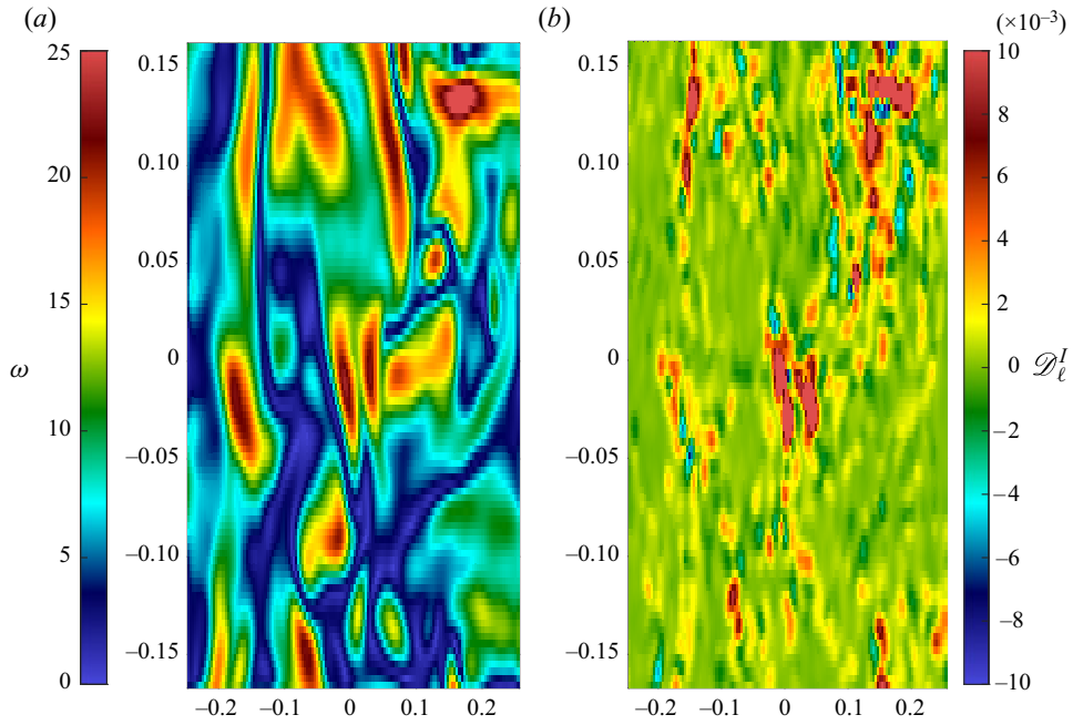
Figure 1. Visualization of the vorticity amplitude \omega (a) and \mathcal{D}_\ell^l (b) for \ell = 3.2\eta for the case T-4 of table 1 in a plane containing the cylinder's axis.
