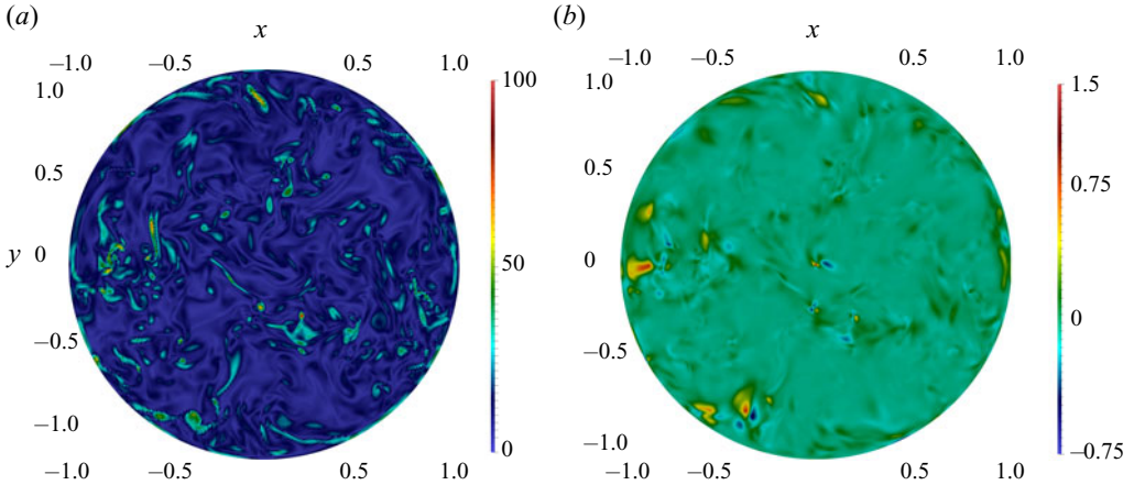
Figure 2. Visualization of the vorticity amplitude of \omega (a) and \mathcal{D}_\ell^l (b) for \ell = 8\eta on a plane containing the centre perpendicular to the cylinder's axis from the DNS of table 1.
