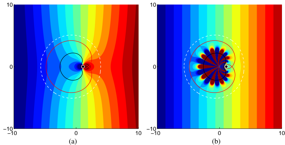
FIG. 2: Real part of the total field with the quasistatic cloaking device (a) inactive and (b) active in the s plane. The color scale is linear from -10 (dark blue) to 10 (dark red) and the scatterer appears in black.
