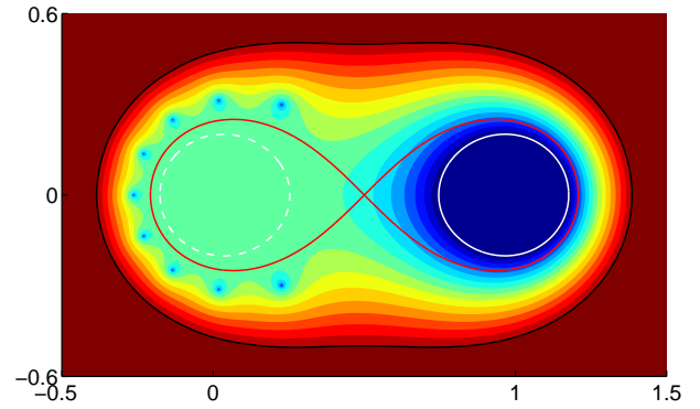
FIG. 1: Magnitude of the Hermite polynomial h(z) for \delta_* = 1 and degree n = 10 . The color scale is logarithmic from 0.01 (dark blue) to 100 (dark red).
