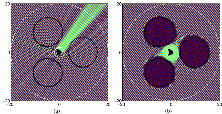
FIG. 3: Real part of the total field with the Helmholtz cloaking devices (a) inactive and (b) active. The color scale is linear from -1 (dark blue) to 1 (dark red) and the axis units are \lambda .
